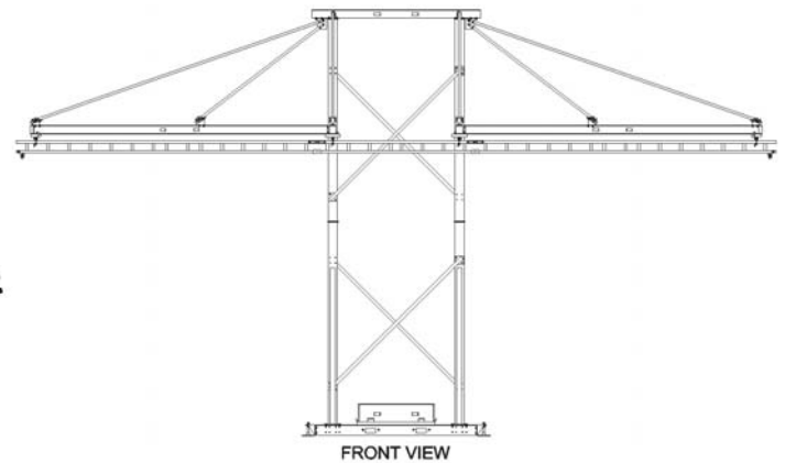
FRONT VIEW
